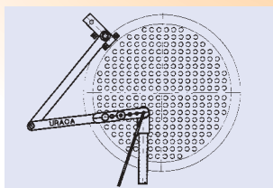
Adjustable device which can be fixed on the heat exchanger with or without bore holes.
